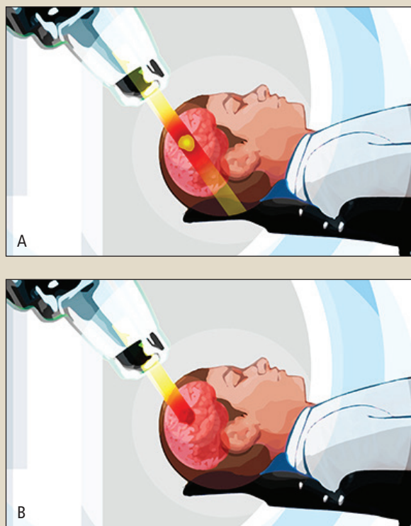
Figure 1: Photon therapy versus proton therapy. Representation of (A) conventional radiotherapy and (B) proton beam therapy. Note the difference in extraneous irradiation to the surrounding tissue. Proton therapy deposits most of its energy on the target and has a zero exit dose. Images courtesy of University Hospitals Cleveland Medical Center.
