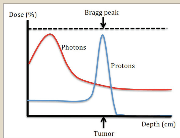
Figure 2: Dose deposition for photon and proton beams as a function of depth. Bragg curve outlining the penetration depth of protons, which eventually reach a maximum dosage at a specific depth (tumor) and then abruptly decrease to zero to spare healthy tissues. Note that even after traveling the distance to the tumor, conventional radiation still requires a relatively higher radiation dosage, potentially damaging surrounding healthy tissues.
